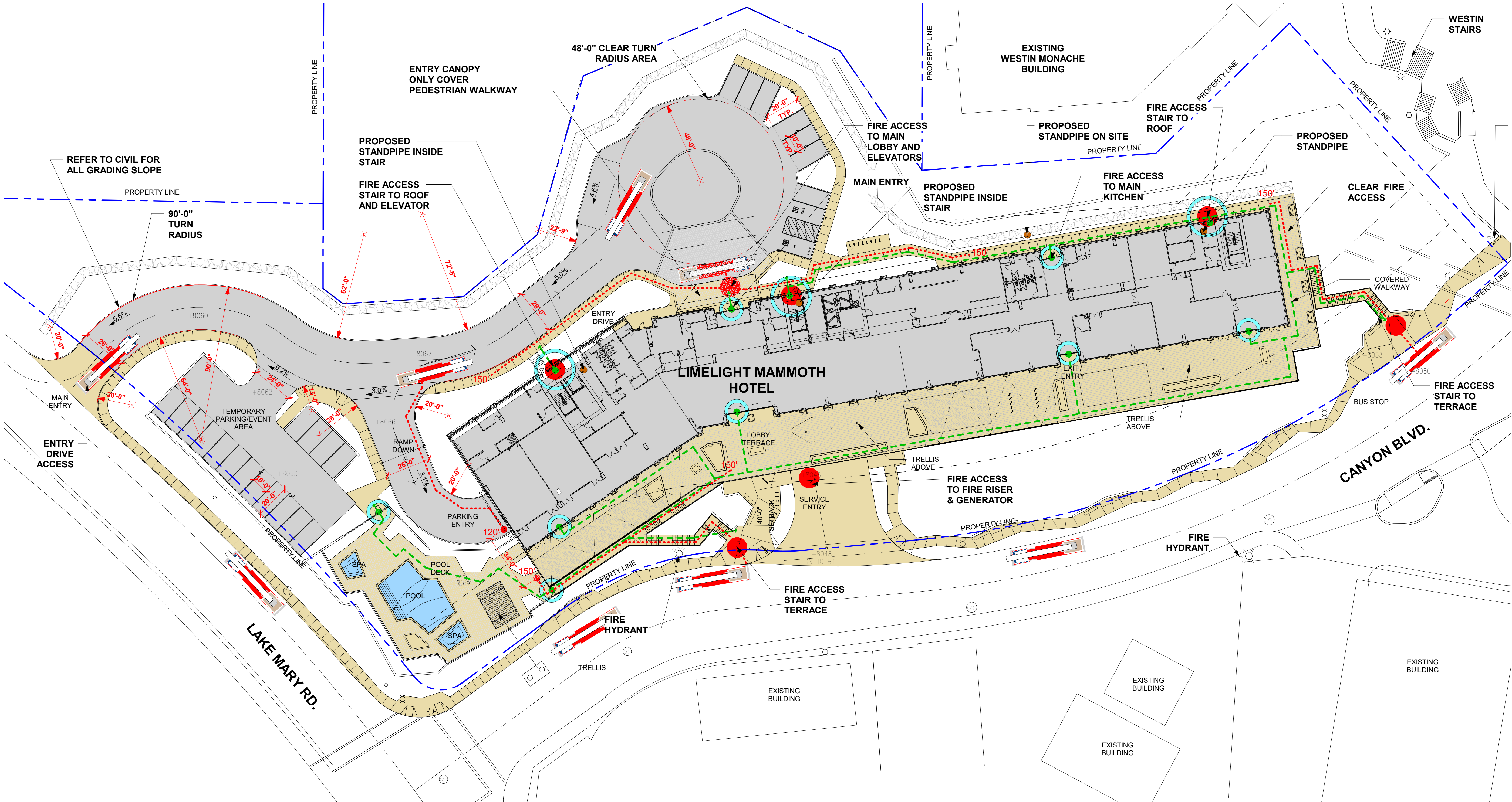
1 FIRE DEPARTMENT SITE ACCESS PLAN 1" = 30'-0"
